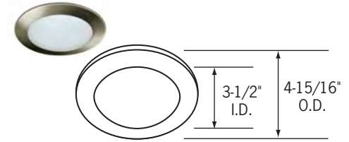
CTR2011FR-(NK, P) Flat Frosted Glass Lens Shower Light All steel construction. (3) heat treated spring steel mounting clips. 1/8" thick heavy duty polyethylene sponge gasket. Wet location listed.
