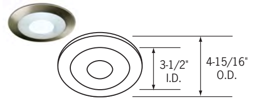
CTR2011-PH-(NK, P) Flat Frosted Glass Lens Shower Light with Clear Pin Hole All steel construction. (3) heat treated spring steel mounting clips. 1/8" thick heavy duty polyethylene sponge gasket. Wet location listed.
