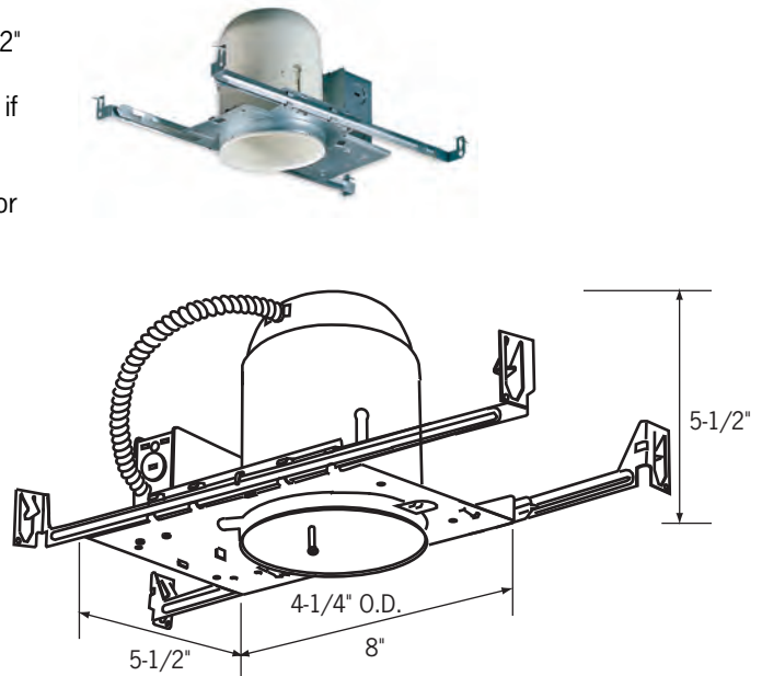
Ceiling Opening: 4-3/4" Plaster Frame: 8" x 5-1/2"
