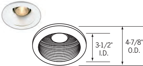
CTR2001-P Black Baffled Downlight CTR2001W-P White Baffled Downlight
