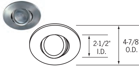
CTR2007-(P, B, NK) Surface Adjustable 28° vertical adjustment. All steel construction. (3) heat treated spring steel mounting clips. Lamp retaining sweep spring clip. PAR20 Lamp only.
