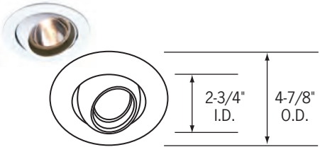
CTR2008-P Eyeball 30° vertical adjustment. All steel construction. (3) heat treated spring steel mounting clips.
